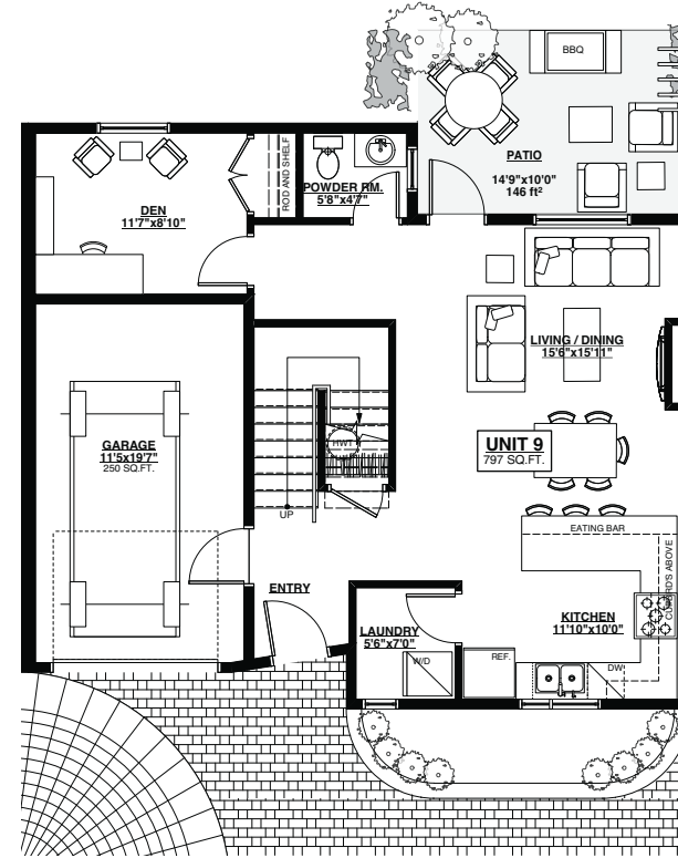
Main Floor 797 Sq Ft
