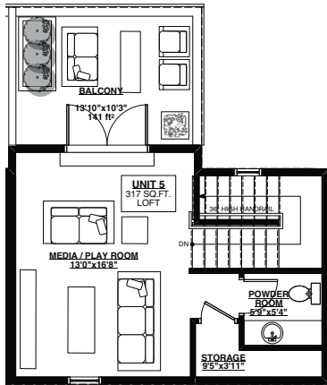
Third Floor 317 Sq Ft
