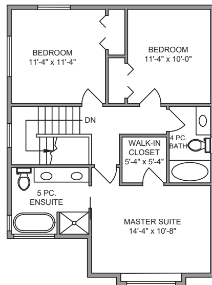
Upper Floor 710 SQ FT
