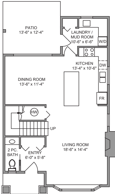
Main Floor 866 SQ FT
