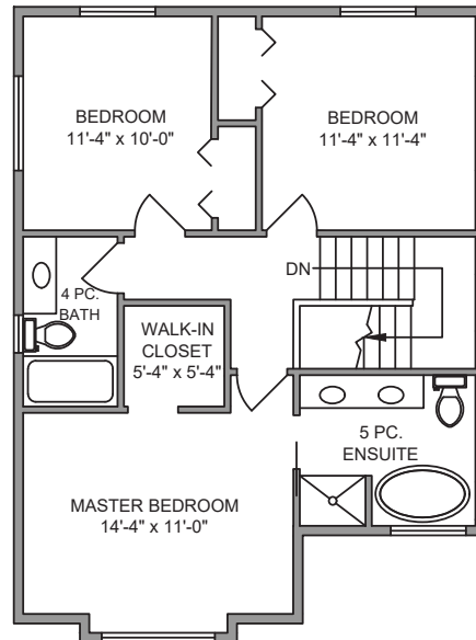
Upper Floor 710 SQ FT
