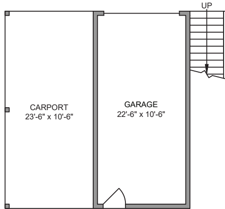
Coach Main 237 SQ FT
